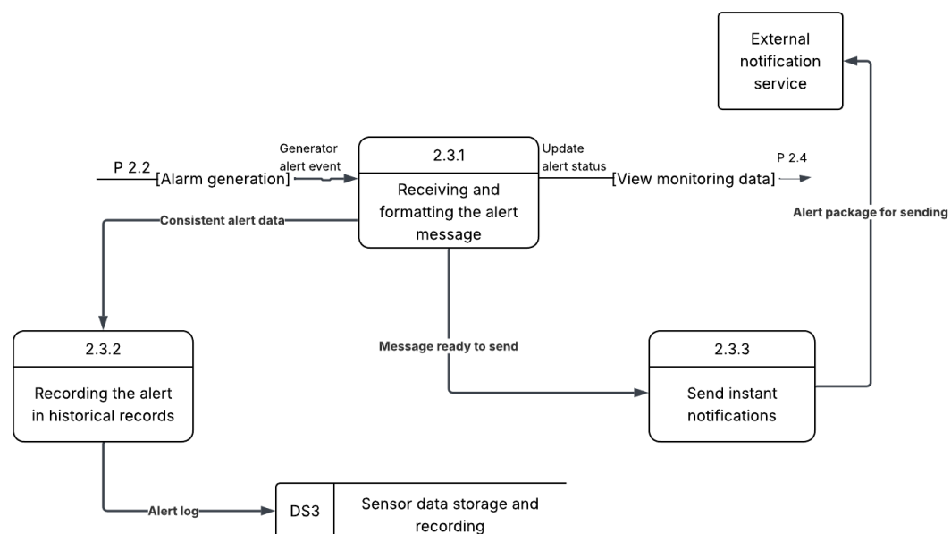
Figure 21 Data Flow Diagram - Level 2 (p2.3) Alerts and notifications management
