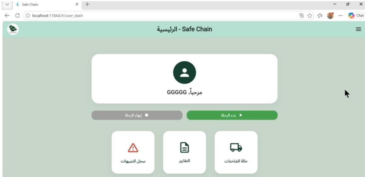
Figure 95 User Screen
