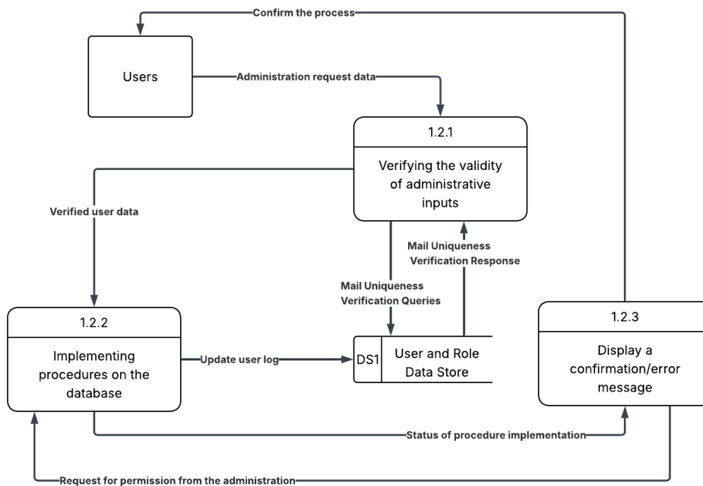
Figure 17 Data Flow Diagram - Level 2 (p1.2) Accounts and Roles Management
